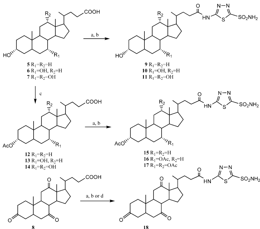
Scheme 1. (a) Ethyl chloro formate, N -methyl morpholine, THF; (b) 4 , reflux; (c) \text{AcCl} , rt; (d) \text{SOCl}_2 , 4 , THF.
